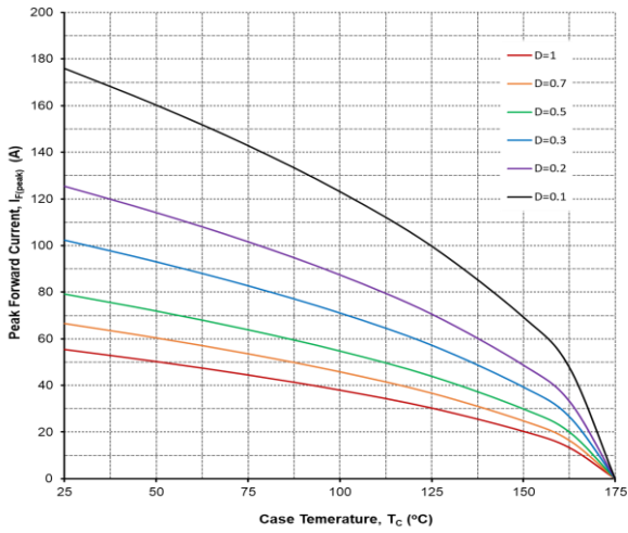
Figure 7. Peak Forward Current vs. Tc
